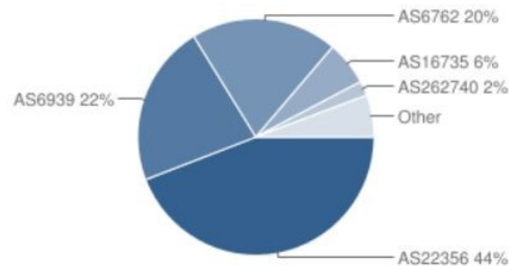
AS264144 IPv6 Peers
